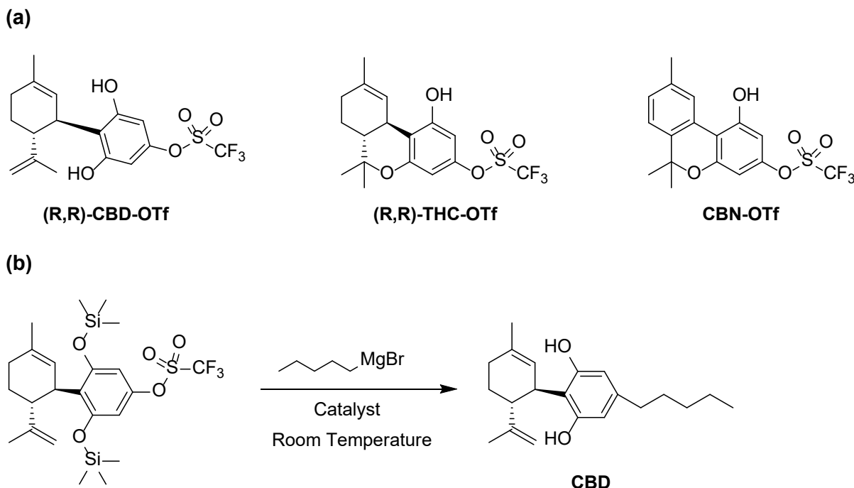
Fig. 1. (a) Cannabinoid precursors (b) catalytic preparation of CBD.
