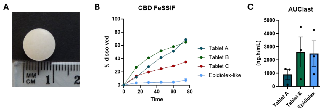
Figure 2. A: Representative tablet form of ART12.11 containing 100 mg CBD. B: FeSSIF CBD dissolution profiles from prototype tablets and an Epidiolex-like solution. C: AUC of ART12.11 tablets and Epidiolex in dogs
